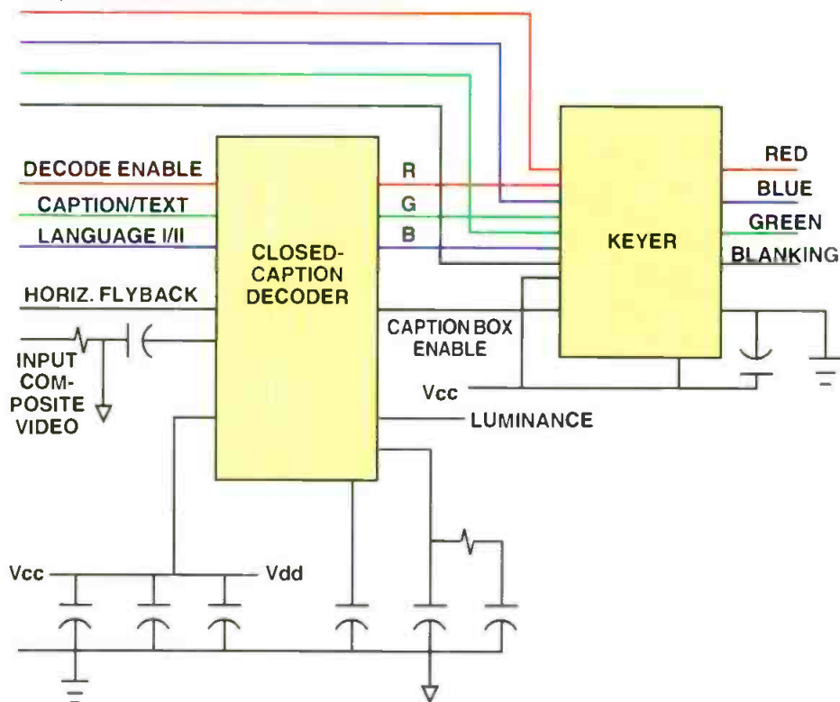
Figure 3. A schematic illustrating interconnections for a Z86128 closed-caption control device. A minimal number of components are used in filters for PLL and device power, as well as coupling for the composite video.
